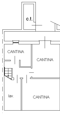
Piano 1S h = 2.40
